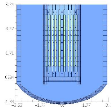
Figure 4. Scheme of ICARE IRIS reactor nodalization of the RPV and core [15].
