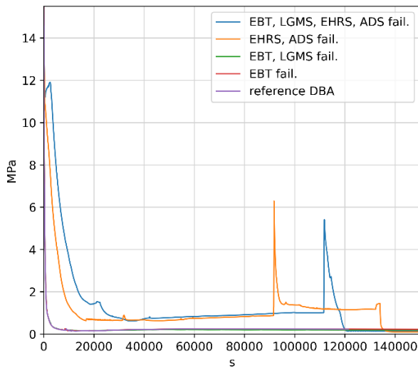
Figure 7. PCS pressure (PRZ).
