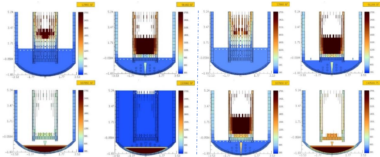
Figure 11. ASTEC - ICARE mask of core degradation evolution for the ADS st-1 and EHRS failure scenario.
