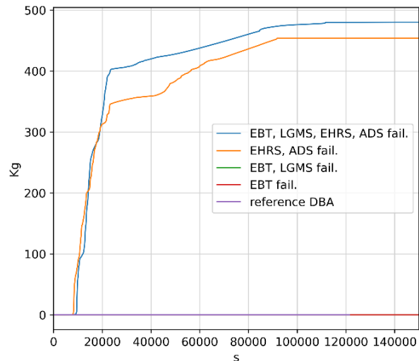
Figure 10. Total hydrogen mass production.
