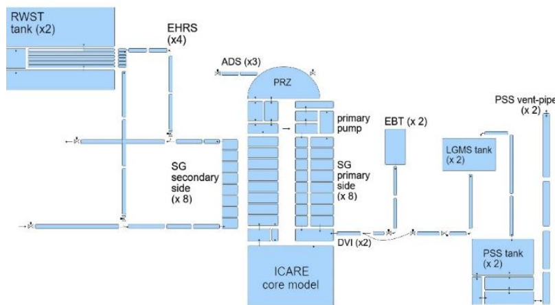
Figure 3. Scheme of CESAR IRIS reactor nodalization of the PCS, secondary coolant system and passive safety systems [15].
