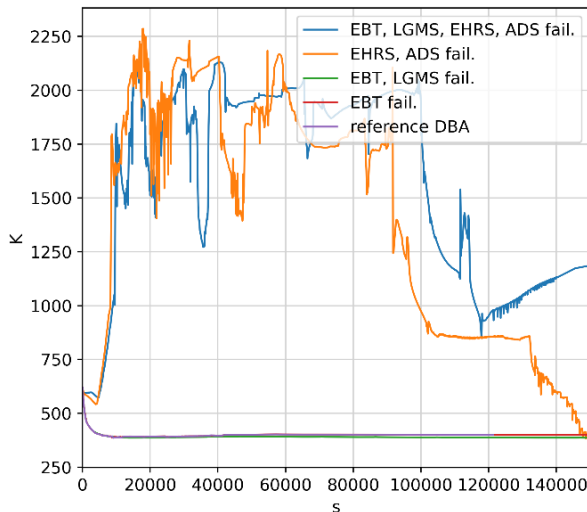
Figure 9. Core outlet temperature.
