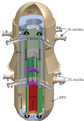
Figure 1. IRIS integral reactor vessel layout [10]
