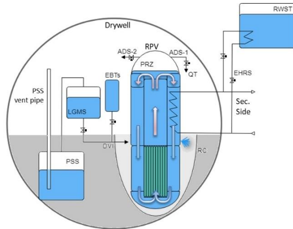
Figure 2. Scheme safety systems for a generic IRIS reactor (for the sake of simplicity, only one line is reported for redundant systems) [12].
