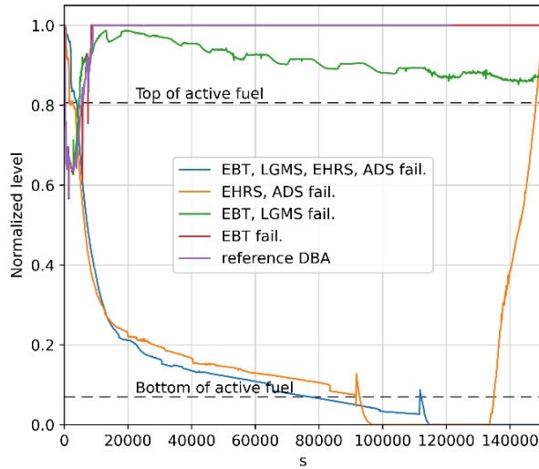
Figure 5. Normalized value of averaged collapsed level in the core (upper and lower core plates elevations taken as reference).
