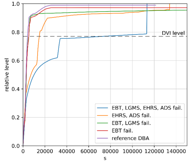
Figure 6. Normalized value of water level in the RC, with respect to the RC total elevation.
