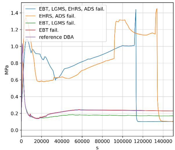
Figure 8. Containment pressure.
